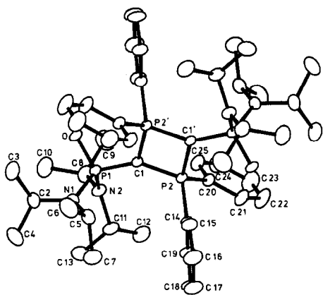
Figure 1. ORTEP plot of \underline{9a} . The size of the vibrational ellipsoids represents a 33% probability
