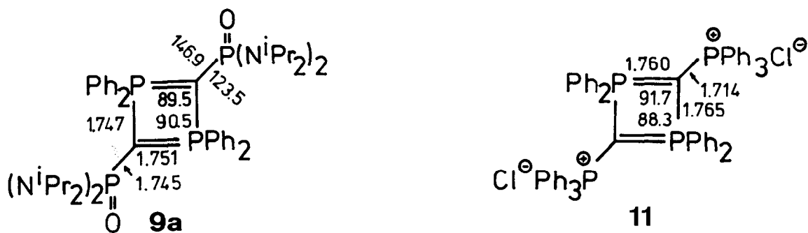
Figure 2. Comparison of bond lengths ( \text{\AA} ) and angles ( ^\circ ) in 9a , 11 and 12 . 9a : Esd's are 0.002-0.003 \text{\AA} and 0.1-0.2 ^\circ ; P-C(phenyl) 1.817(3), 1.813(3); P-N 1.687(3), 1.672(3) \text{\AA} .
